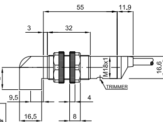
M12 CONNECTOR
